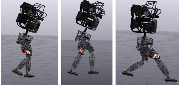
Fig. 6. A sequence of states from the executed trajectory as the robot uses its arm to help climb up onto the step in less than 3 seconds.
