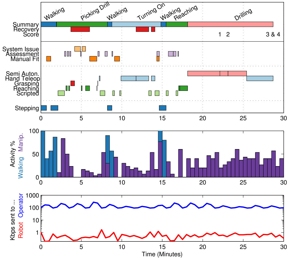
Figure 17: Analysis of the Drill Task. Top: Analysis of operating time. From top to bottom: summary of task components, time spent recovering from mistakes, and times when points were scored; time spent primarily stationary while the operators considered the situation and manually fit objects; manipulation modes; and time spent stepping. Center: Portion of time the robot spent moving integrated over 30 second intervals. Bottom: Data transmission rates from robot to operator (blue) and vice versa (red).
