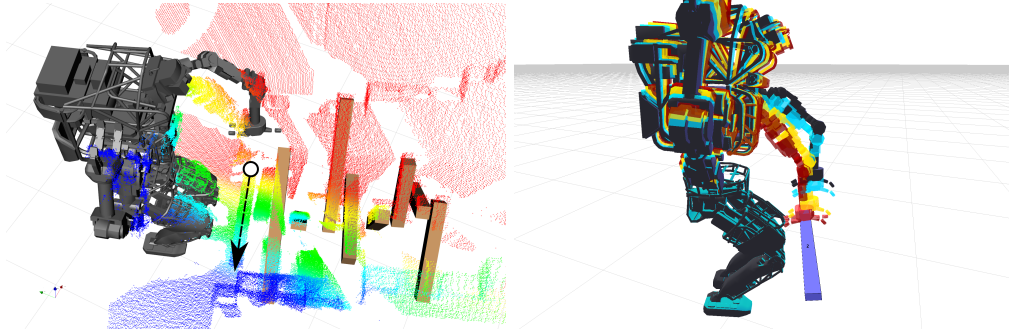
Figure 12: A fitting algorithm produces an affordance that can be used to plan a reach motion. Left: A line annotation (arrow) defines a search region that is used by a segmentation algorithm to fit a 2”x4” board affordance to the 3D point cloud data. Right: An end effector goal placed on the board affordance is used to compute a reaching plan.
