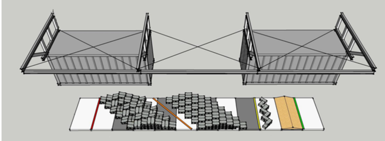
Figure 18: The DRC Trials Terrain Course (graphic credit: DARPA). Execution was from right to left. The cinder blocks on the left side were tilted at angles of 20–40 degrees.
