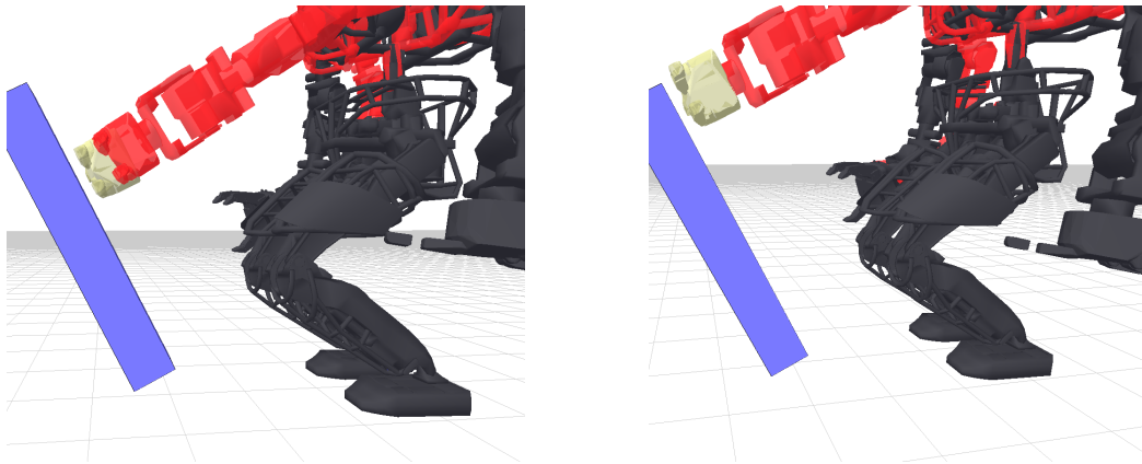
Figure 9: Relaxation of reaching plans to the affordance (blue) by the robot (grey). Left: a pre-grasp reaching goal (yellow) just reachable (red) after automatic relaxation in position and orientation (by 2 cm and 3 degrees respectively in this case). Right: if the operator was unhappy with the relaxation, the reaching goal could be manually repositioned until precisely reachable. Here the planner is simultaneously solving for the 6 joints of the arm and the 3 back joints.
