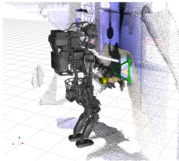
Figure 16: Top left: head camera view of poker used to press drill's power button. Top right: visualization of the nominal plan to reach all drill target points in the triangle. Bottom right: head camera view provides situational awareness to operator as robot executes drilling plan. Bottom left: Robot avatar and RGB point cloud visualization with affordance models of the drill and triangle target.
