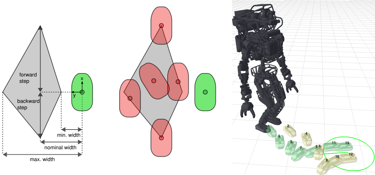
Figure 10: Left: A simplified representation of the kinematic reachability region for footstep placement. Given a fixed position and orientation of the right foot, we compute a polyhedral region defined by parameters min width , max width , etc. into which the next position of the left foot must be contained. In practice, this polyhedron is represented in four dimensions: x , y , z , and yaw, but only x and y are drawn here. Center: several example locations for the left foot (red) relative to the right foot (green). Right: A complete footstep plan from the robot’s position to the target position and orientation showed by the green circular marker. In this particular plan, the robot steps forward, then to the side, then backward in order to reach the goal.
