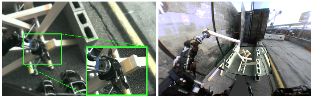
Figure 13: Left: an example of foveation during the debris task to enhance the operator’s situational awareness without drastically impacting bandwidth. The operator selects a region of interest on a low-resolution image to request a high-resolution sub-image. Right: a first-person combined view stitches the head camera image with the left and right fish-eye chest camera images. The operator can use the mouse to zoom and look in all directions for superior situational awareness.
