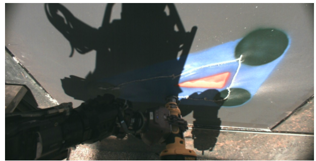
Figure 16: Top left: head camera view of poker used to press drill's power button. Top right: visualization of the nominal plan to reach all drill target points in the triangle. Bottom right: head camera view provides situational awareness to operator as robot executes drilling plan. Bottom left: Robot avatar and RGB point cloud visualization with affordance models of the drill and triangle target.
