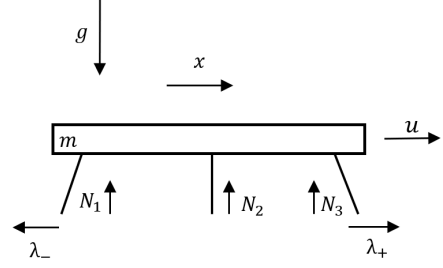
Fig. 13. Regulation task of a 3 legged table.
