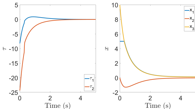
Fig. 16. Simulation results for 2D simple manipulation example. The forces applied to the box ( \tau ) are smooth even though u is not, due to the low-pass filter model.
